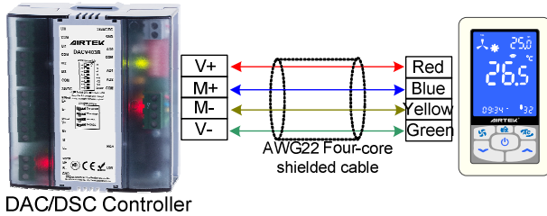
Fig. 1 Wiring diagram of MST32V operation panel
