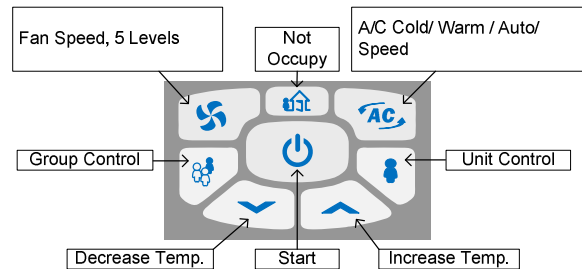
FIG.2 NST32V Key diagram
