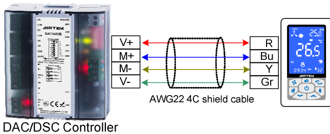
FIG.1 NST32V Wiring diagram
